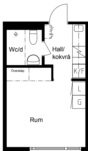
PLAN 3
