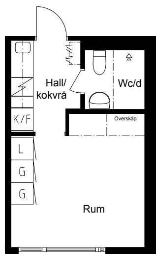
PLAN 2,
