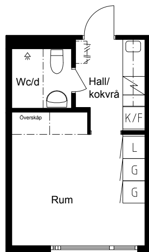
PLAN 3,
